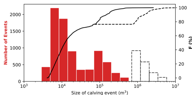
Figure 6. Cumulative distribution function (right axis) and histogram (left axis) showing size-frequency relationship of all detected calving events observed subaerially at Store for 23 days from July 5 to July 27, 2017. Dashed black bars show posited actual size of full-thickness calving events which is estimated to be nine times greater than the subaerially observed fraction because the glacier is near floatation. Dashed black line shows the cumulative distribution function based on the inferred actual size (dashed bars) rather than the observed red bars ( >7 \times 10^4 \text{ m}^3 ). Compare with Figure 5 above.
