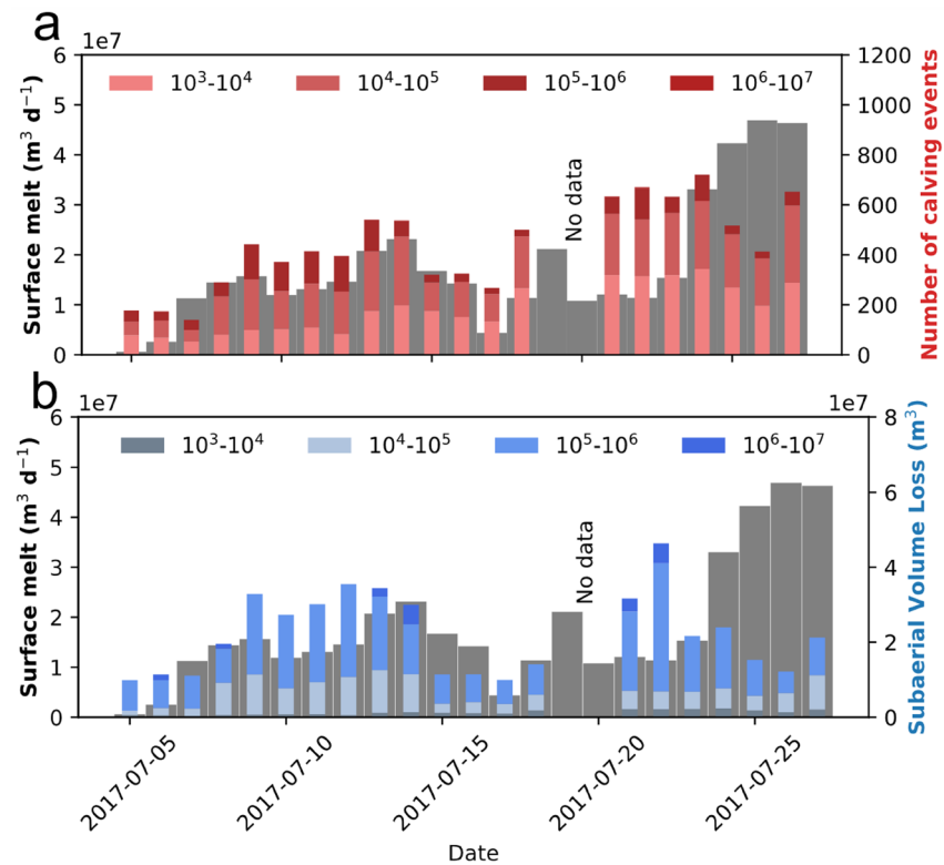
Figure 8. Time series of surface melt from RACMO 2.3p2 data (gray bars, left axis) and TRI-derived calving events (colored bars, right axis). (a) Calving event frequency (red bars) and (b) calving volumes (blue bars). TRI, terrestrial radar interferometer.
