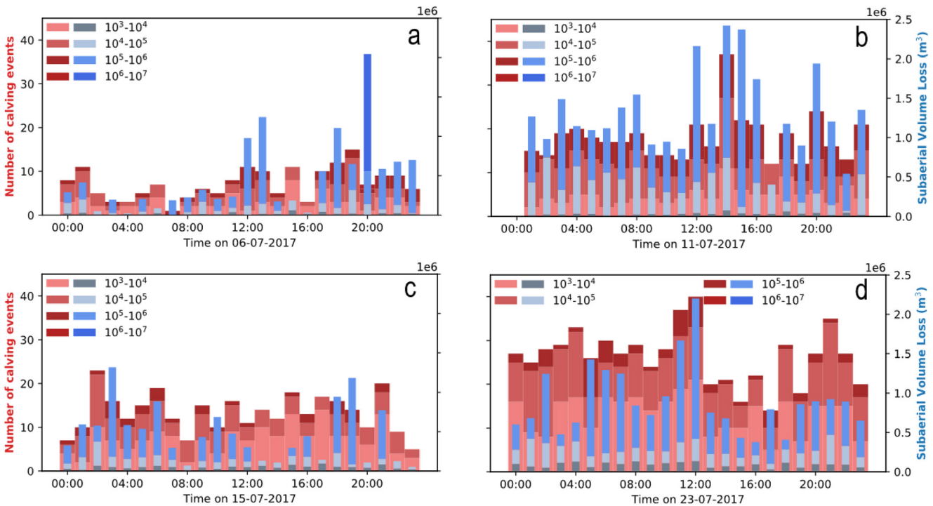
Figure 9. Time series of calving binned by hour from (a) 06/07/2017 (before mélange breaks up), (b) 11/07/2017 (high calving activity following mélange break-up), (c) 15/07/2017 (reduced calving activity), and (d) 23/07/2017 (renewed high calving activity).
