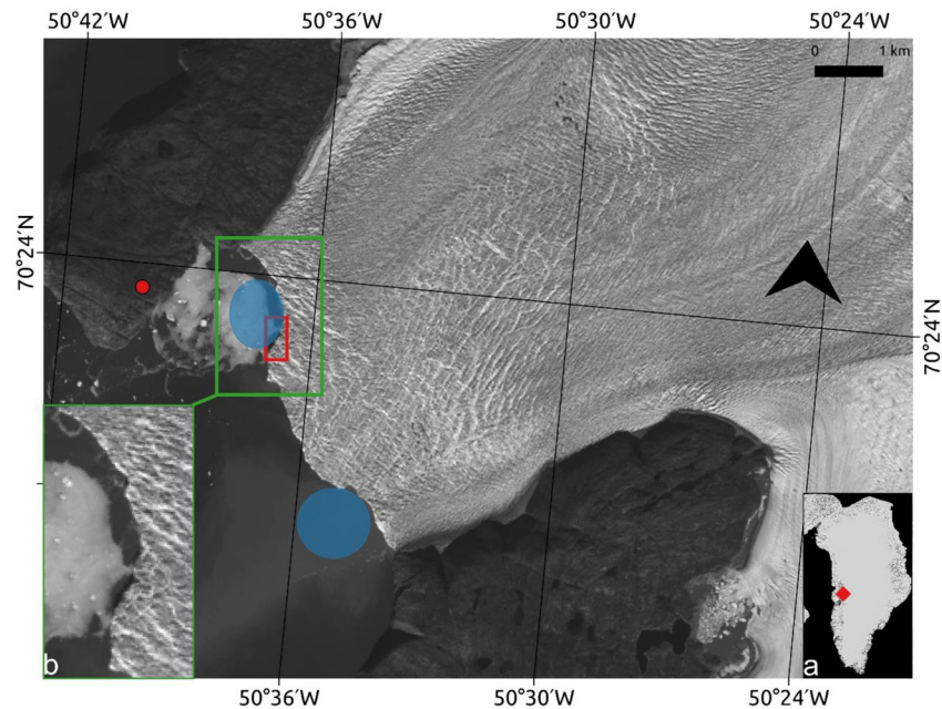
Figure 1. Location of Store Glacier (inset (a)) and location of TRI and time-lapse camera (red circle). The study area is outlined in green (inset (b)). The red rectangle represents the zoomed area in Figures 2 and 3, and the blue circles show the two regions where surfacing plumes are commonly observed in the time-lapse imagery. Background image from Landsat 8, acquired on October 10, 2016.
