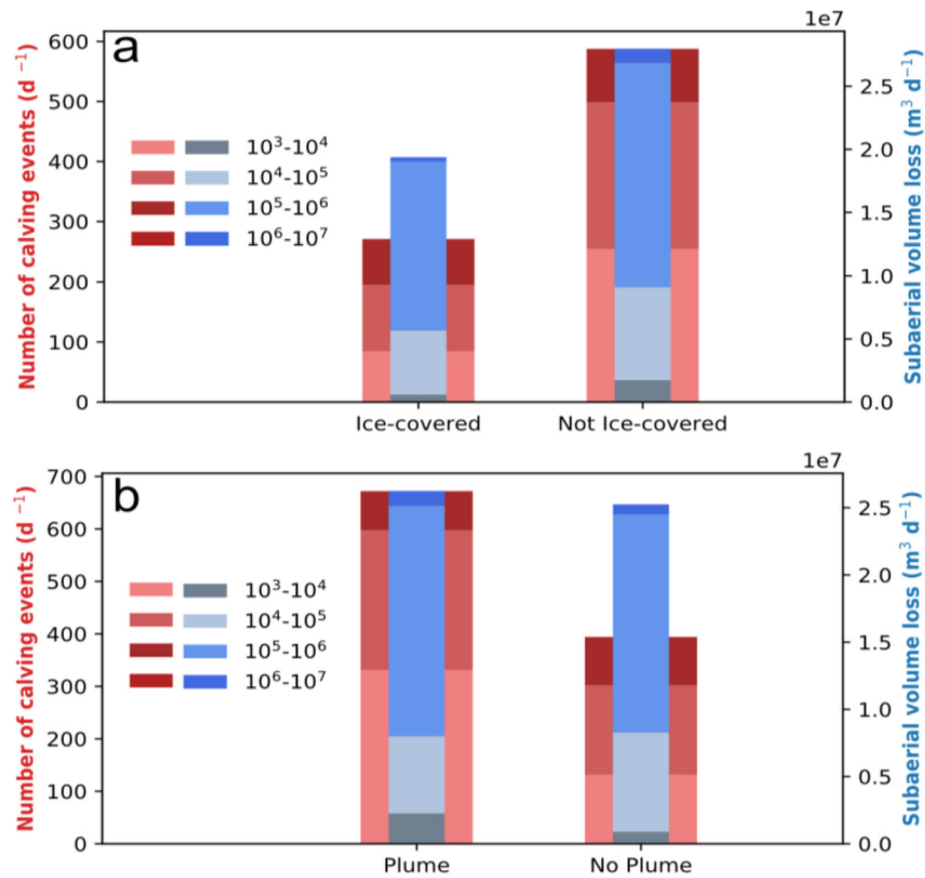
Figure 10. Calving event counts and volumes during times when (a) mélangé is present compared to when it is not, and (b) when plumes are visible compared to when they are not. Note how mélangé presence suppresses calving activity and how plume presence increases the frequency of smaller and mid-sized calving events.
