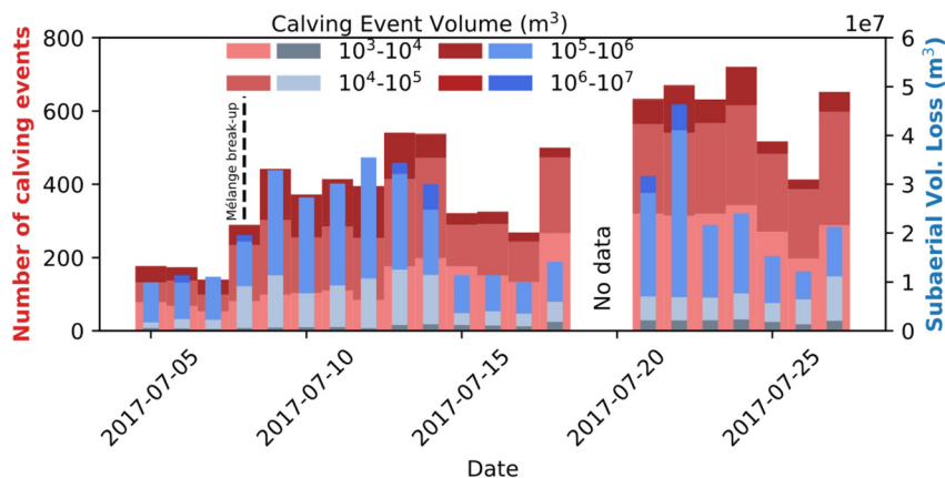
Figure 7. Time series of calving events at Store. Bars stacked by volume of event. Daily counts are shown by thick red bars; cumulative volumes by the inner blue bars. Note how calving activity increased on July 8 when the proglacial mélange broke up.
