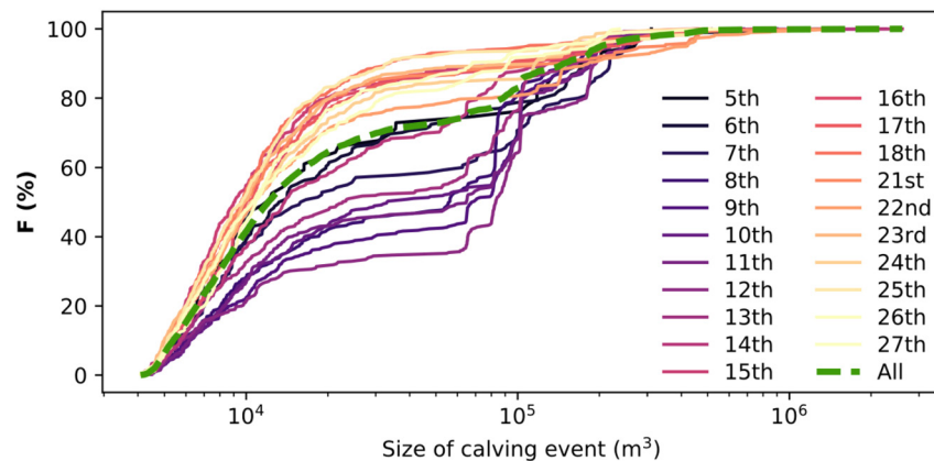
Figure 11. Cumulative distribution function for calving events observed from July 5 to 27, 2017, with colored lines denoting distribution on specific days and dashed green line showing the overall distribution. Notice how days earlier in the observation period cluster below the overall average distribution, whereas those later in the period cluster above it.
