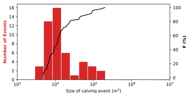
Figure 5. Cumulative distribution function (right axis) and histogram (left axis) of frequency-magnitude relationship of single set of calving events at Store for the 12 h from 22:17 12/07/17 to 10:15 13/07/17 considered in the UAV validation exercise. Compare with Figure 6 below. Size refers to the observed subaerial volume. UAV, unmanned aerial vehicle.
