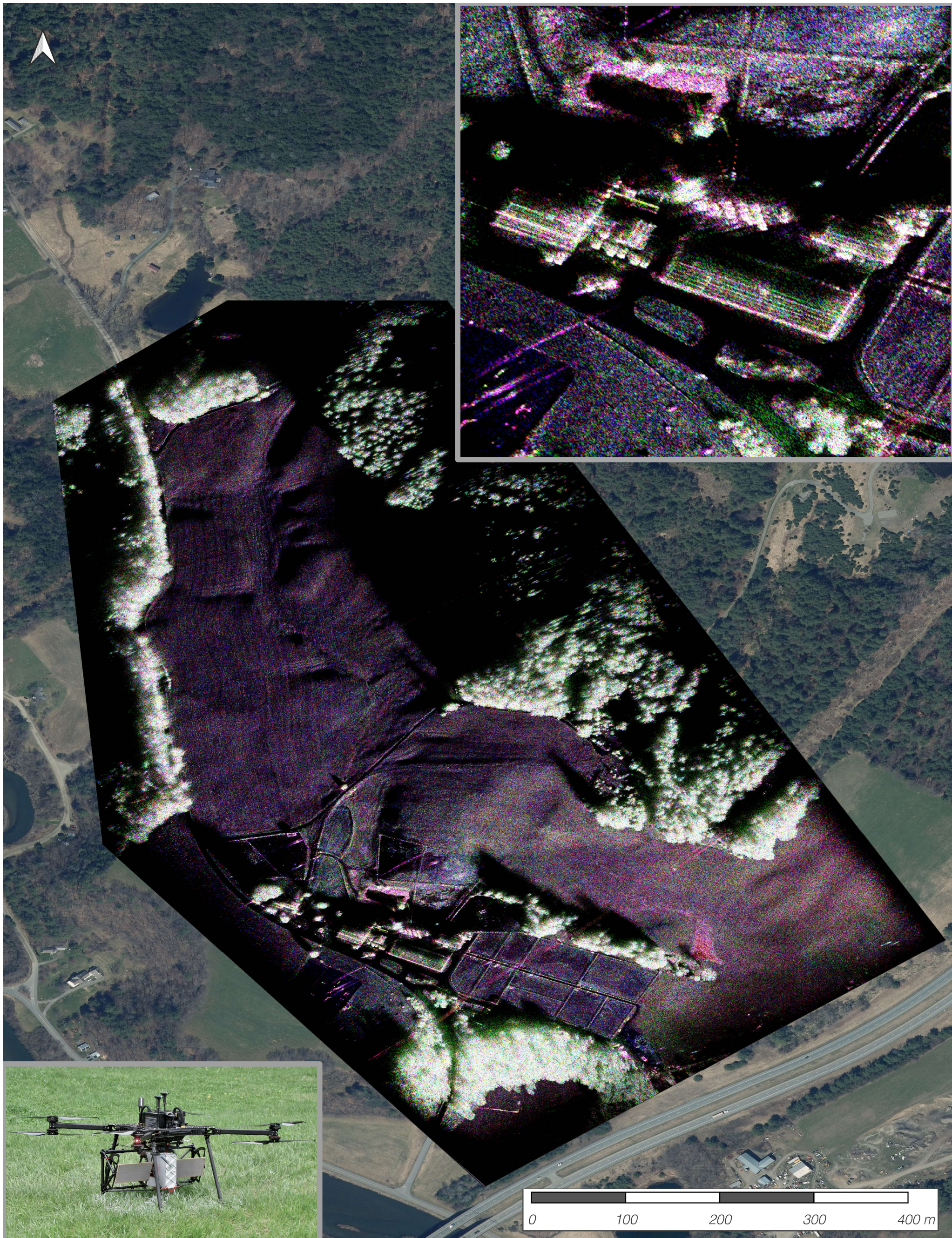
Gamma S-Band SAR, 400MHz bandwidth, < 40cm resolution: fully polarimetric Pauli SAR image taken from a Harris HX8 octocopter drone
